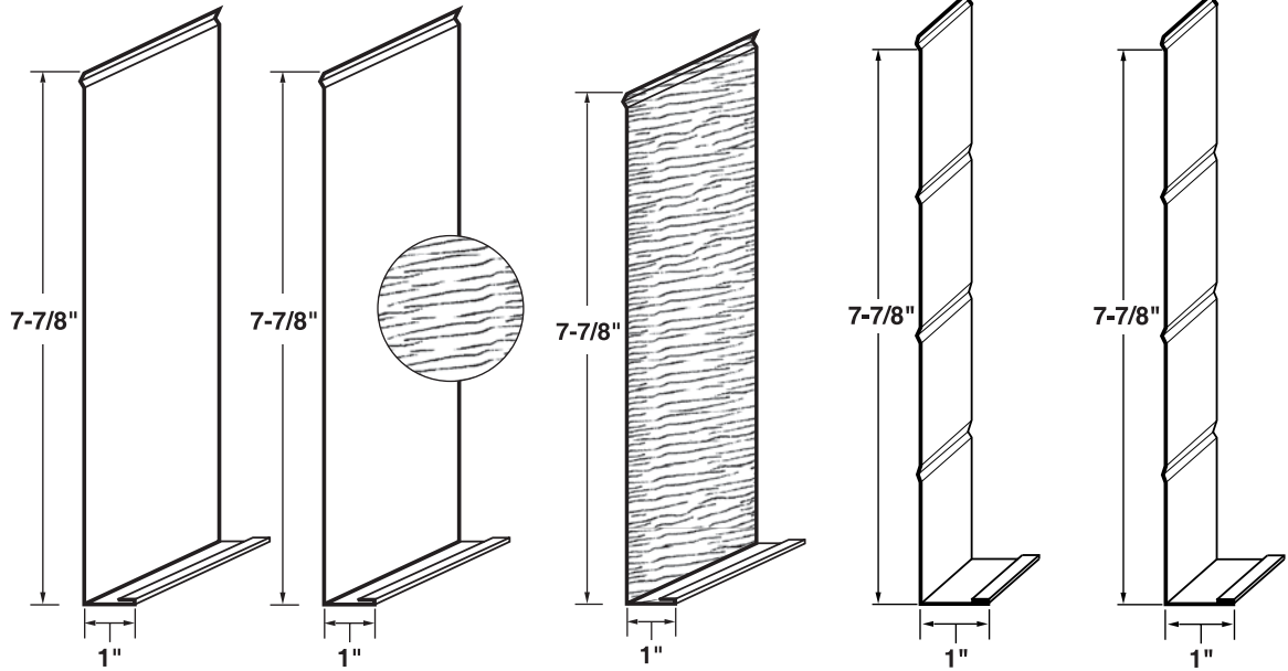
ENVOY SMOOTH FASCIA TRIM 4", 6", 8", 10" .024 NOMINAL
